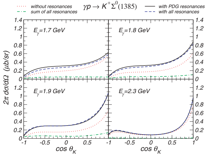
FIG. 5. (Color online) Differential cross sections for \gamma p \rightarrow K^+ \Sigma^0(1385) at E_\gamma = 1.7, 1.8, 1.9, and 2.3 GeV with the inclusion of resonances. The dash-dash-dotted line is the sum of the resonance terms. See the text for the details.
