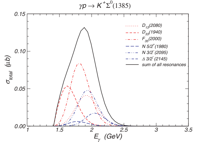
FIG. 4. (Color online) Contributions from various resonances to the total cross section for \gamma p \rightarrow K^+ \Sigma^0(1385) .
