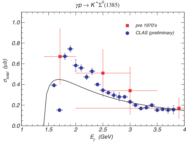
FIG. 2. (Color online) Total cross sections for \gamma p \rightarrow K^+ \Sigma^0(1385) without resonance contributions. The pre-1970s data are from Refs. [11–13] and the preliminary data of CLAS Collaboration are from Ref. [5].
