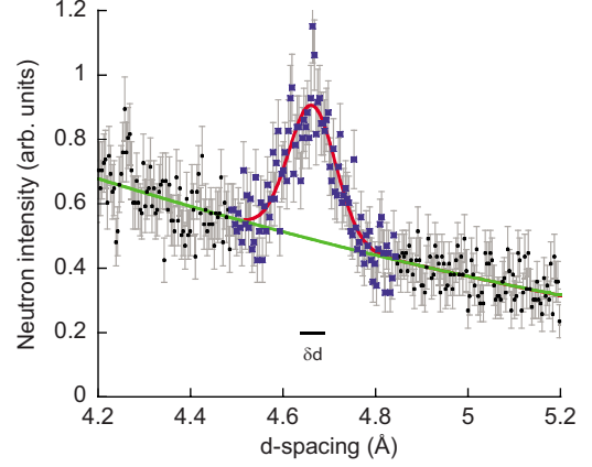
FIG. 10. (Color online) The (100) Zn 0.30 Fe 0.70 F 2 AF Bragg reflection profile at 6 K showing the intensities (blue squares) and fitted background (green curve) whose difference is the integrated intensity of the reflection.
