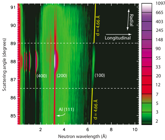
FIG. 6. (Color online) Neutron intensity image (neutrons counted in a bin with dimensions 0.005 Å by 0.066°, scale at right) vs 2θ and λ. (h00)-type Bragg reflections are labeled. The intensity within the dashed box was integrated along contours of constant d spacing to form the diffraction pattern in Fig. 7. A contour of constant d spacing (d=4.66 Å) is shown by the yellow line.
