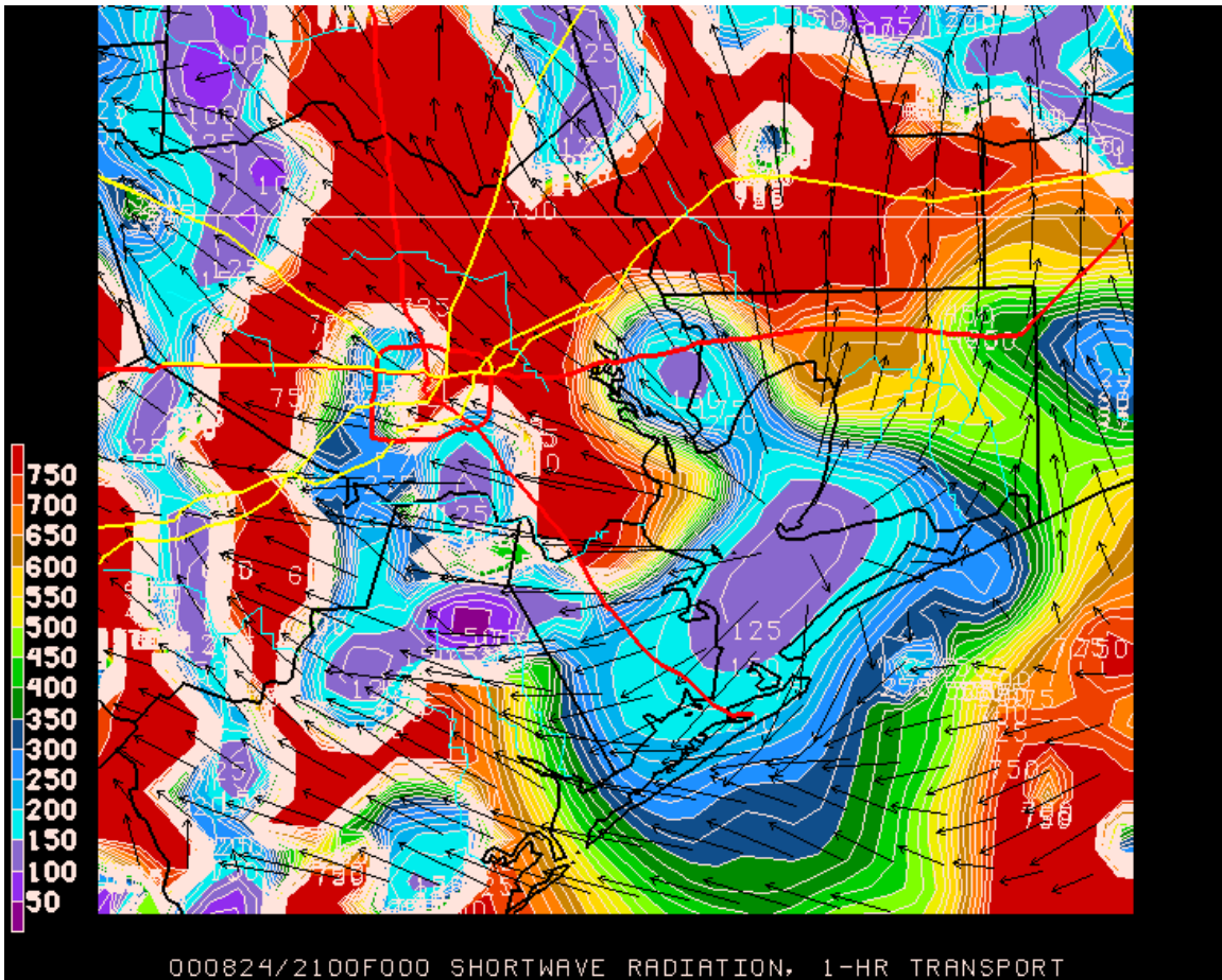
Figure 10: Incoming solar radiation ( \text{W}/\text{m}^2 ) and surface wind vectors (length equal to one-hour air parcel motion), dec30grid4 run, 2100 UTC August 24.
