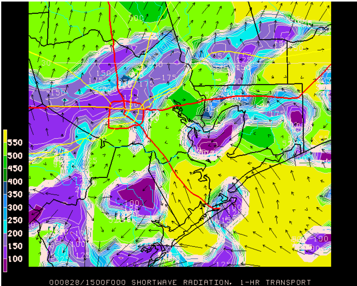
Figure 12: Incoming solar radiation (W/m 2 ) and lowest sigma level wind vectors (length equal to one-hour air parcel motion), dec16grid4 run, 1500 UTC August 28.
