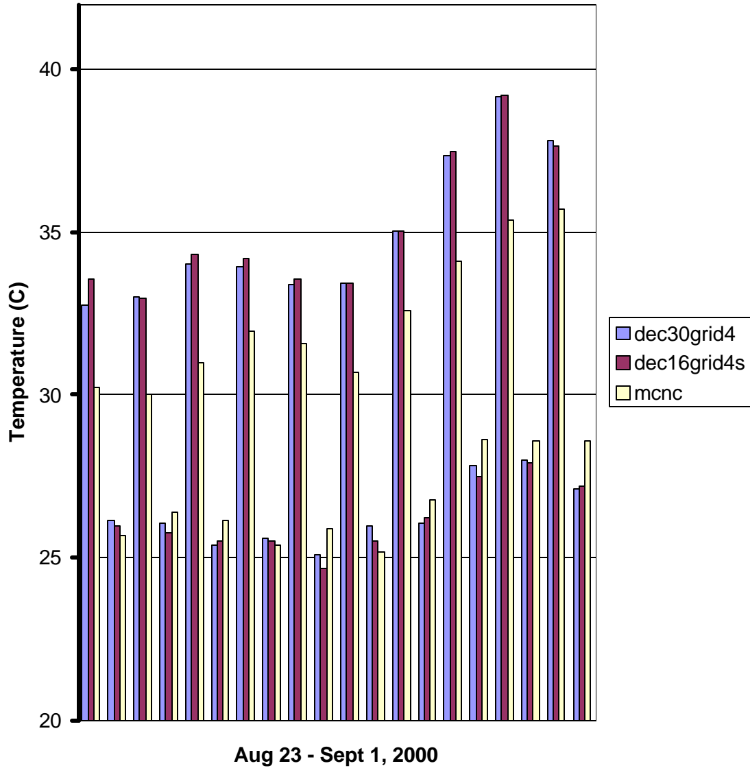
Figure 17: Maximum and minimum temperatures at the 17 m level (TAMU runs) and 19 m level (MCNC run) at seven National Weather Service observing sites in the Houston/Galveston area during the ozone episode.
