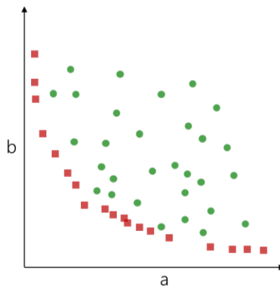
Figure 2.2 Pareto front (red dots) and dominated solutions (green dots)
