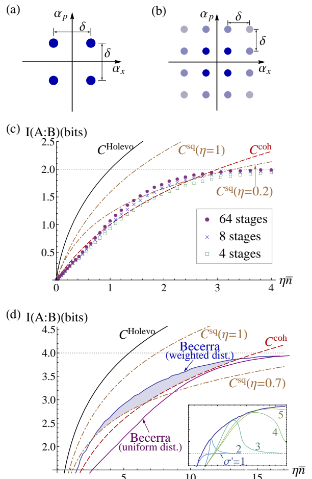
FIG. 3. (a) 4-QAM and (b) 16-QAM with more probable inputs in darker blue. Mutual information with (c) 4-QAM and (d) 16-QAM using the Becerra receiver, which beats all Gaussian schemes in the shaded region. Inset: capacity of Becerra receiver with \sigma' = \{1, 2, 3, 4, 5\} (thin curves) and optimal \sigma (thick curve). Horizontal dotted line represents the maximum possible capacity 2-bits (4-bits) for 4-QAM (16-QAM).
