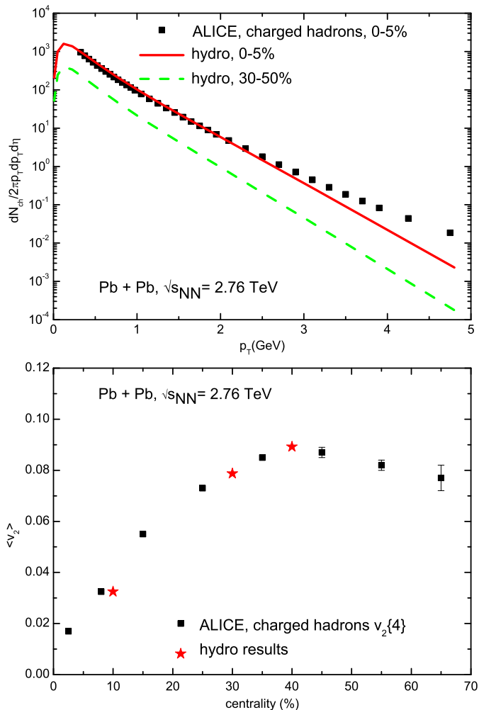
Fig. 1. (Color online.) Hydrodynamic fits of charged-hadron spectra and inclusive elliptic flow to ALICE data [45,46] using our updated AZHYDRO tune.
