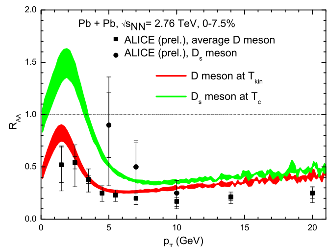
Fig. 4. (Color online.) D - versus D_s -meson R_{AA} for 0–7.5% central Pb+Pb, compared to ALICE data [27]. The bands indicate the charm-shadowing uncertainty.
