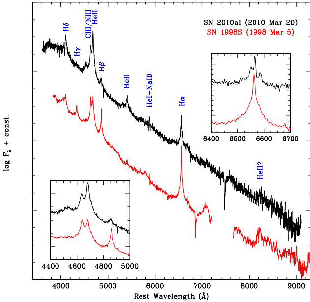
Figure 7. Comparison between the earliest optical spectra of SN 2010al and the Type IIn SN 1998S (Fassia et al. 2001). The two spectra are reddening- and redshift-corrected. The inserts show a blow up of the region between 4400 and 5000 Å (bottom-left) and the region of H \alpha (top-right) in the two spectra.
