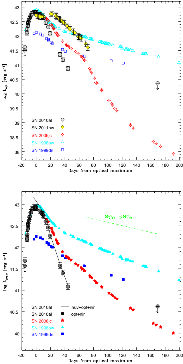
Figure 5. Quasi-bolometric light curves of the Type Ib/c SNe 2006jc, 2011hw and 2010al compared with those of the normal SN Ib 1999dn (Benetti et al. 2011) and the broad-lined Ic SN 1998bw (Patat et al. 2001, and references therein). Top: Pseudo-bolometric light curves for the SN sample have been computed by integrating the fluxes in the optical bands only. Bottom: The pseudo-bolometric light curves have been obtained by integrating the broadband fluxes in the optical and NIR domains. In the case of SN 2010al, also an uvoir curve obtained including the near-UV contribution is shown (solid line), although limited to phases later than -3.7 days from maximum. Error-bars have been reported for SNe 2010al and 2011hw, and account for uncertainties in the distance and the reddening estimates, spectral energy distribution fitting and photometric errors.
