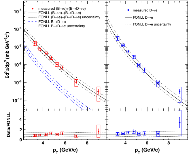
FIG. 17 (color online). Invariant cross section of electrons ( \frac{e^+ + e^-}{2} ) from bottom (upper left) and charm (upper right) decay, together with the ratio of the corresponding measurements to the FONLL predictions for bottom (lower left) and charm electrons (lower right). The solid circles are experimental measurements. The error bars and the boxes are, respectively, the statistical and systematic uncertainties. The solid and dotted curves are the FONLL predictions and their uncertainties. The dashed and dot-dashed curves are the FONLL prediction for B \rightarrow D \rightarrow e , i.e. electrons from the decays of D mesons which in turn come from B meson decays.
