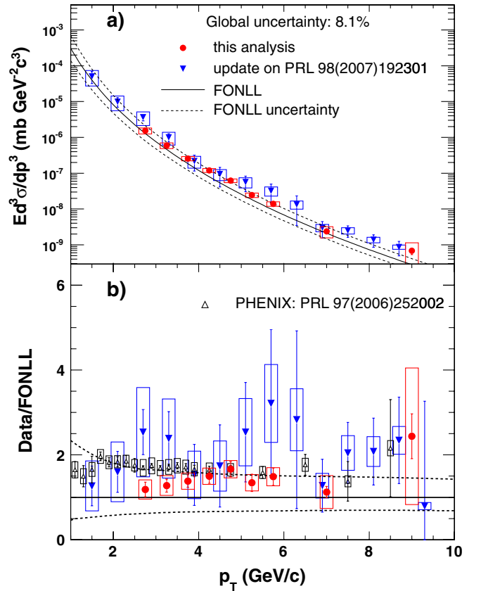
FIG. 16 (color online). (a) Invariant cross section of nonphotonic electron production ( \frac{e^+e^-}{2} ) in p + p collisions from this analysis (closed circles) after combining results from Run2005 and Run2008. The published STAR result [16] (closed triangles) is also shown. (b) Ratio of data over FONLL [2] from all measurements at RHIC including PHENIX results [17] (open triangles).
