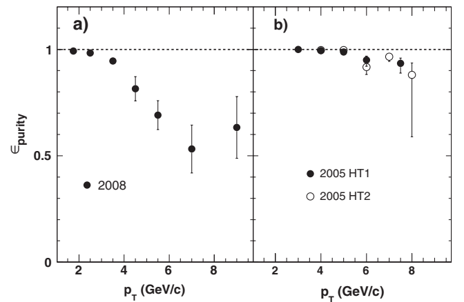
FIG. 6. Purity of the inclusive electron sample as a function of p_T in data from (a) Run2008 and (b) Run2005. The 2008 result is from combined data sets of all different high-tower triggers. The 2005 results for the two different high-tower triggers, i.e. HT1 (closed circles) and HT2 (open circles), are plotted separately.
