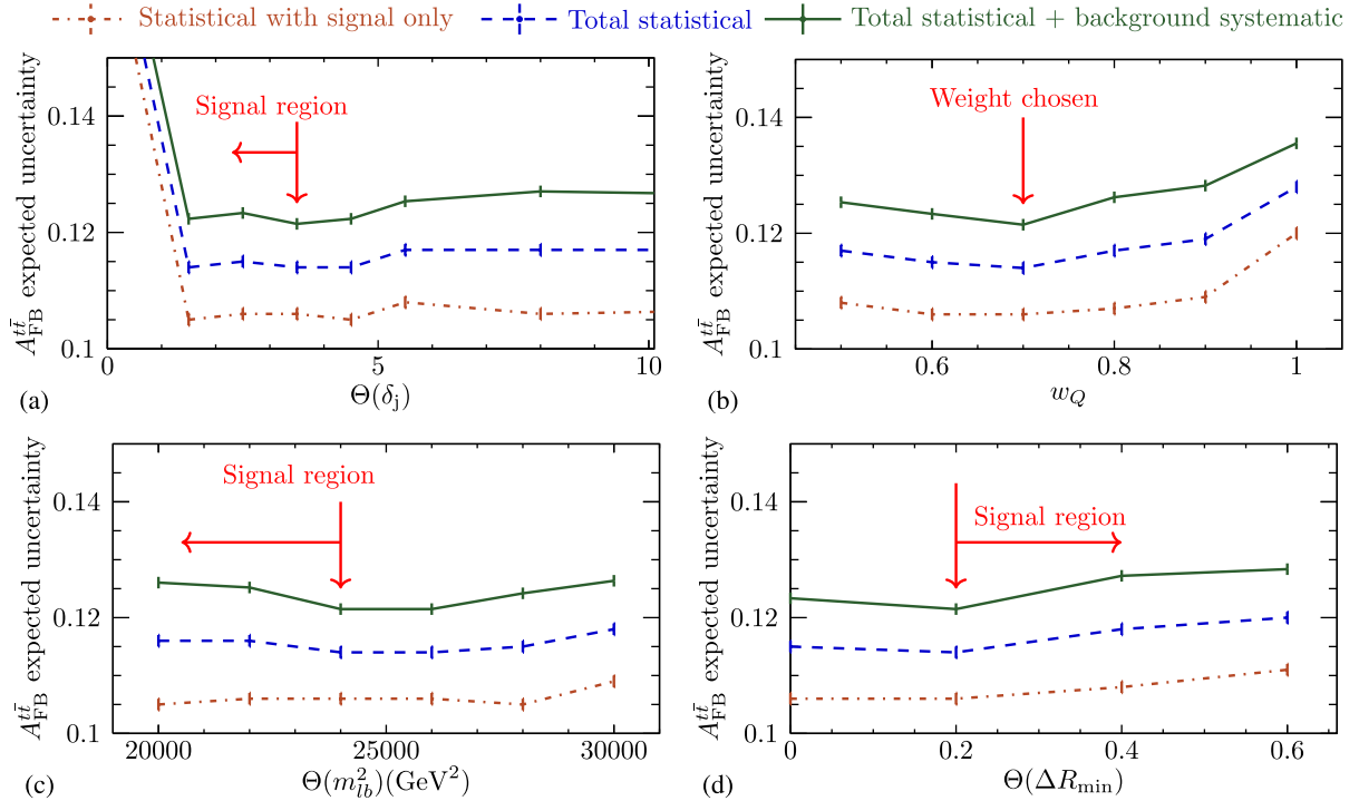
FIG. 2. Expected uncertainties as functions of the four optimization parameters, \Theta(\delta_j) (a), w_Q (b), \Theta(m_{bb}^2) (c), and \Theta(\Delta R_{\min}) (d). In each plot is shown the statistical uncertainty for signal only (dash-dotted line), statistical uncertainty for signal and backgrounds (total statistical uncertainty, dashed line), and the quadrature sum of the total statistical uncertainty and the background systematic uncertainty (solid line). The optimal values are based on the minimum point of the green solid line, as marked with the vertical arrows on the plots, and summarized in Table I. For each plot, all other optimization parameters are held at their optimal values.
