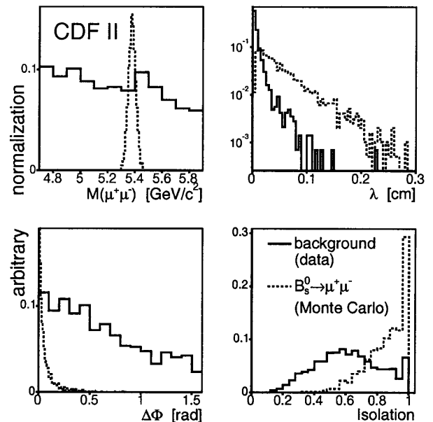
FIG. 1. Arbitrarily normalized distributions of the discriminating variables for events in our background-dominated data sample (solid line) compared to Monte Carlo B_s^0 \rightarrow \mu^+\mu^- events (dashed line).
