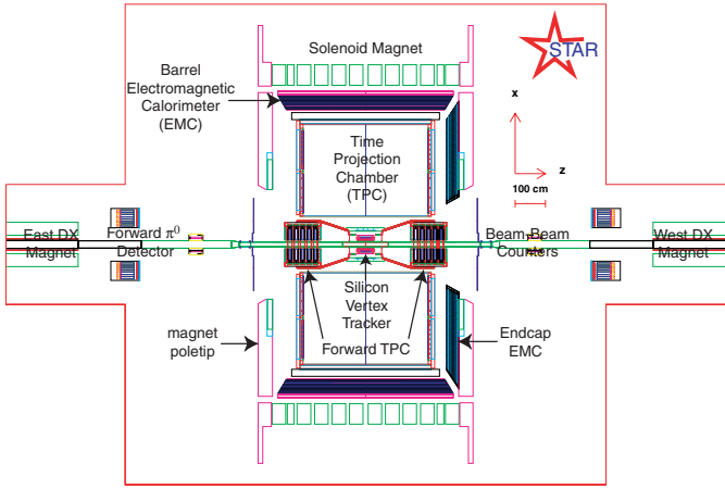
Fig. 1. Layout of the Solenoidal Tracker at RHIC [10]
