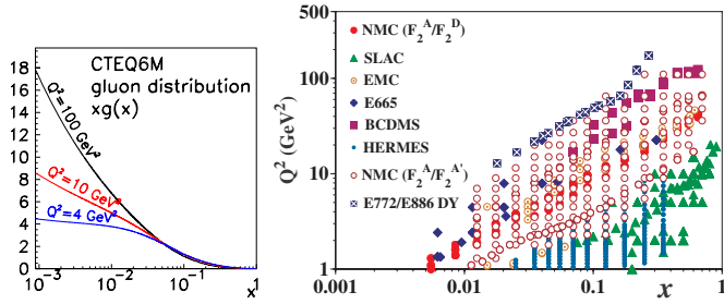
Fig. 2. Left: The gluon distribution in the proton [4]. Note the rapid rise in xg(x) for x < 0.01 , a discovery made at HERA based on studies of deep inelastic scattering (DIS), using electron(positron)+proton collisions at \sqrt{s}=300 GeV [12, 13]. Right: Values of DIS kinematic variables x and Q^2 where nuclear data from fixed-target DIS experiments at much lower \sqrt{s} constrain the nuclear gluon density for x > 0.02 [6, 7]
