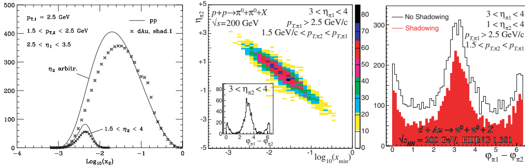
Fig. 3. Left: pQCD calculation of \pi^0 - \pi^0 production at large \eta in pp and d+Au collisions at \sqrt{s_{NN}}=200 GeV [35]. The distributions integrate to d\sigma/dp_T in units of pb/GeV. The smallest x values are probed when \pi^0 - \pi^0 pairs are detected at large \eta . Middle: PYTHIA [36] simulation for \pi^0 - \pi^0 production at large \eta in pp collisions at \sqrt{s}=200 GeV. The \eta of the associated \pi^0 is strongly correlated with the x value of the soft parton involved in the partonic scattering. Right: HIJING simulation for \pi^0 - \pi^0 production at large \eta in d+Au collisions at \sqrt{s}=200 GeV. Compared to the pp simulations, the peaks in \Delta\phi = \phi_{\pi_1} - \phi_{\pi_2} corresponding to elastic parton scattering, sit atop a background from other mechanisms for particle production
