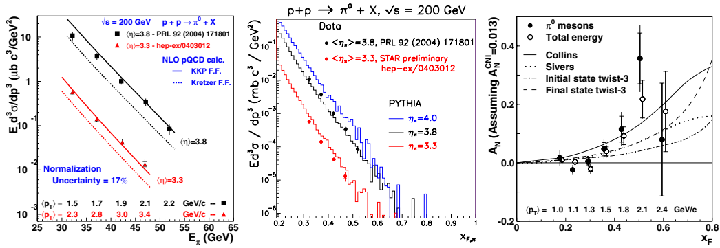
Fig. 5. Left: Invariant cross sections for inclusive \pi^0 production at large rapidity in pp collisions at \sqrt{s}=200 GeV [11,43] compared to NLO pQCD calculations [27–29]. Middle: The data are compared with predictions from PYTHIA [36]. Right: The analyzing power for \pi^0 production at \langle\eta\rangle=3.8 in pp collisions at \sqrt{s}=200 GeV [11]. The curves are predictions from pQCD models [48,50,52] evaluated at p_T=1.5 GeV/ c
