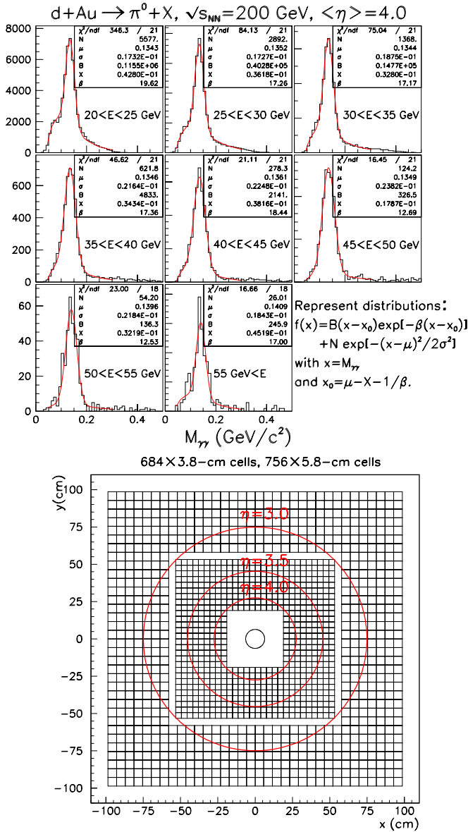
Fig. 6. Top: Di-photon invariant mass distributions from the STAR FPD for d+Au collisions at \sqrt{s_{NN}}=200 GeV at \langle \eta \rangle = 4.0 relative to the incident deuteron beam. Bottom: Layout of the proposed FMS
