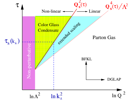
Fig. 4. Diagram showing the boundary between possible “phase” regions in the \tau = \ln(1/x) versus \ln(Q^2) plane [22]. BFKL evolution [23] results in expected exponential growth of the gluon density at fixed Q^2 and increasing \tau . DGLAP evolution is discussed in the text
