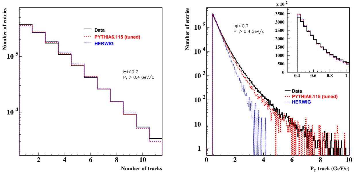
FIG. 10: Distribution of track multiplicity (left) and transverse momentum (right) in the \sqrt{s} = 630 GeV minimum bias sample. The inset in the right plot shows the low P_T portion of the spectrum on a linear scale.
