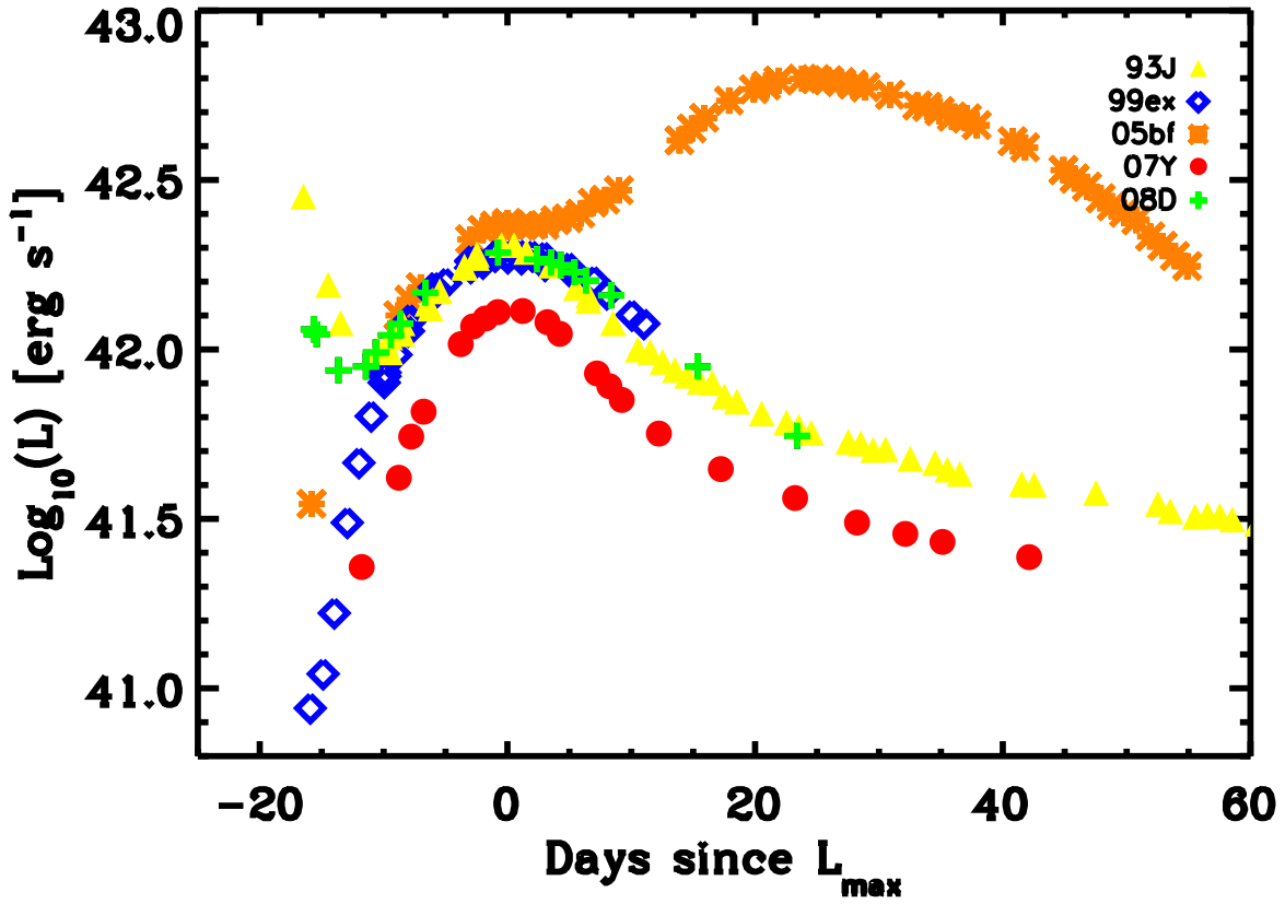
FIG. 7.— Comparison of the bolometric (UVOIR) light curves of SN 2007Y (red filled circles) with the SNe Ib 1999ex (blue diamonds), 2005bf (orange stars), 2008D (green crosses), and the SN Ib 1993J (yellow triangles). A reddening of E(B-V) = 0.112 mag and a distance of 19.31 Mpc have been adopted to place the UVOIR light curve of SN 2007Y on an absolute flux scale. Note that the last four epochs of SN 2007Y do not include any contribution from the ultraviolet.
