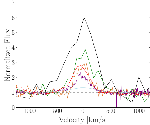
Fig. 14.— Evolution of the He II 4686Å emission. Spectra taken on days 2, 15, 40, 516, 1819 and 1881 are shown in light blue, purple, red, orange, green and black, respectively. The local continuum has been normalized to one by fitting a first order polynomial.
