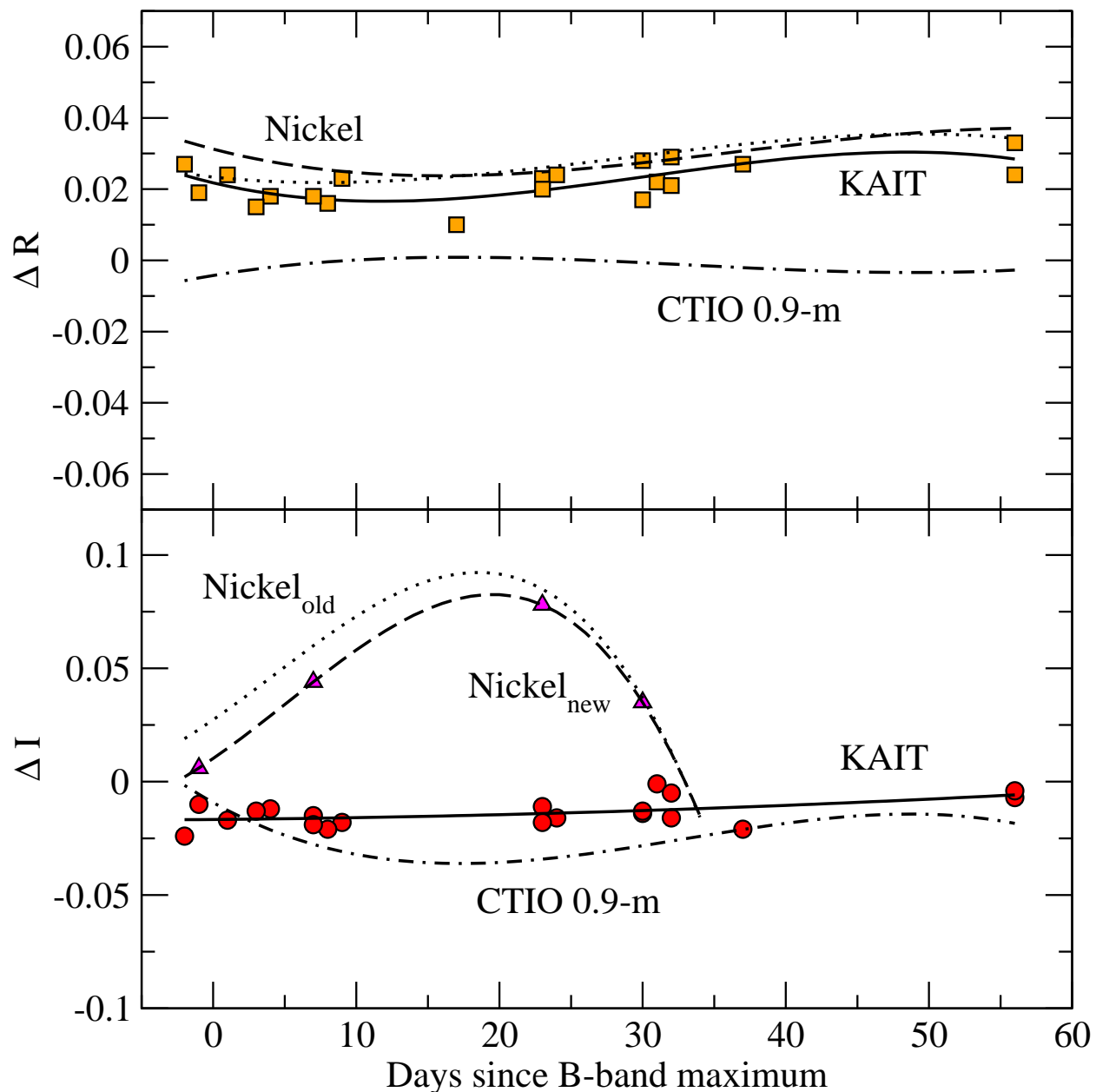
Krisciunas et al. Figure 5. S-corrections for R - and I -band photometry of SN 2001ay. Corrections for the older Nickel 1-m chip are shown as a dotted line; corrections for the new Nickel 1-m chip are shown as a dashed line. For the I -band corrections with the Nickel 1-m filter and both CCD chips used in the camera, we can only use spectra that extend to sufficiently long wavelengths (our Keck spectrum, two spectra taken with the Lick 3-m, and one with the KPNO 4-m). For the Nickel 1-m photometry to match the KAIT photometry, we would need the S-corrections to be a factor of 3 larger than the derived values. S-corrections are added to the photometry to correct it to the filter system of Bessell (1990).
