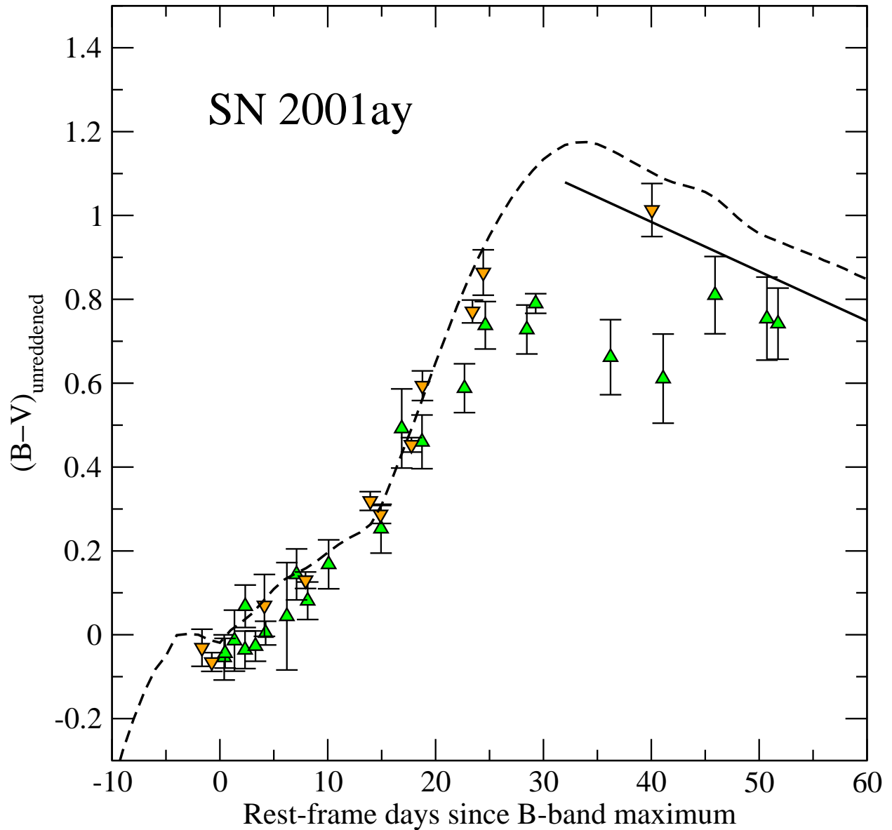
Krisciunas et al. Figure 7. Unreddened B - V colors of SN 2001ay vs. time since B -band maximum. Upward pointing triangles are data derived using image-subtraction templates. Downward pointing triangles represent data derived from aperture magnitudes without template subtractions. The dashed line is the locus from Prieto, Rest, & Suntzeff (2006b) for their most slowly declining object (with \Delta m_{15}(B) = 0.83 mag). The solid line is the commonly used Lira-Phillips locus (Lira 1995; Phillips et al. 1999).
