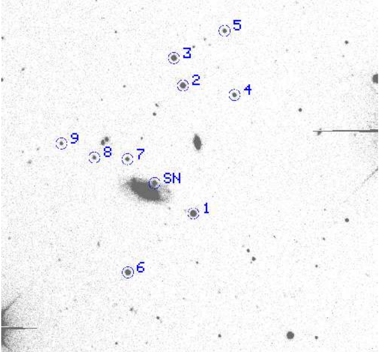
Krisciunas et al. Figure 1. Finder chart for IC 4423, SN 2001ay, and some field stars in our Galaxy. This 7.4' \times 7.4' image is a 200 s V -band exposure obtained on 2001 May 23 with the CTIO 1.5-m telescope. North is up and east is to the left. The SN is located 10.3'' W and 9.3'' N of the galaxy core.
