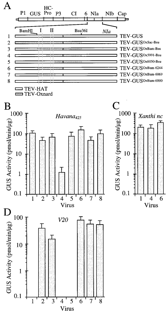
FIG. 5. (A) Diagrammatic representation of chimeric TEV genomes. Vertical boxes delineate locations of clusters I and II as shown in Fig. 4B. (B to D) Systemic infection of Havana 425 (B), Xanthi nc (C), and V20 (D). The number under each bar corresponds to the code for each virus as shown in panel A. GUS activity was quantitated in 2+ leaves at 7 days p.i. Each bar represents the mean \pm standard deviation from eight plants. Note that the scale of the y axis in panels B to D was adjusted to provide the best relative comparison of data within each panel.
