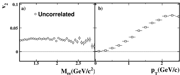
FIG. 18. The dielectron v_2 from the c\bar{c} contribution as a function of M_{ee} and p_T with a completely uncorrelated c and \bar{c} .
