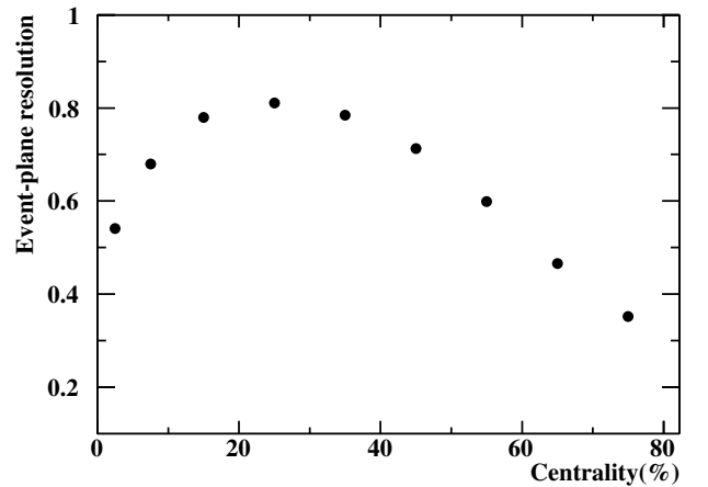
FIG. 13. The event-plane resolution from central to peripheral (left to right) collisions in minimum-bias Au+Au collisions at \sqrt{s_{NN}} = 200 GeV.
