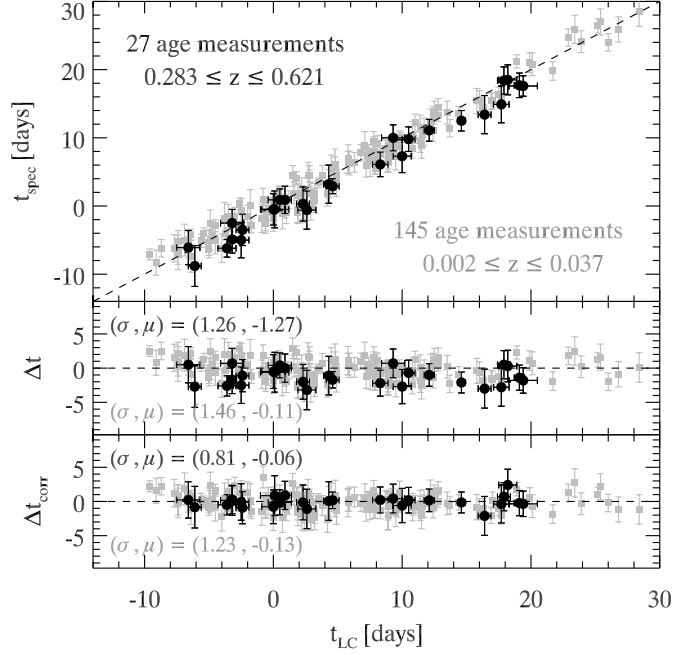
FIG. 10.— Top : Comparison of supernova rest-frame ages (in days from maximum light) obtained from cross-correlation with spectral templates ( t_{\text{spec}} ) and from fits to the light curve ( t_{\text{LC}} ), showing 145 age measurements for the subsample of 22 low-redshift SNe Ia ( gray ). The dashed line represents the one-to-one correspondence between t_{\text{LC}} and t_{\text{spec}} . Middle : Age residuals, \Delta t = t_{\text{spec}} - t_{\text{LC}} . We also indicate the standard deviation ( \sigma ) and mean residual ( \mu ). Bottom : Same as above, where each point has been corrected for the mean offset between t_{\text{spec}} and t_{\text{LC}} .
