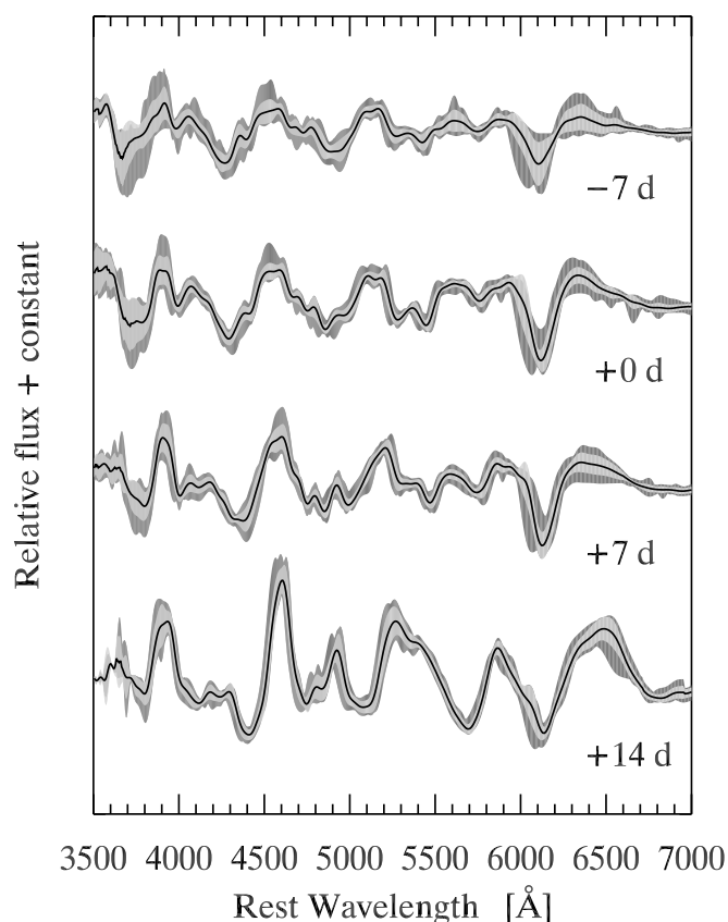
FIG. 2.—Standard ( light gray ) and maximum ( dark gray ) deviation from the mean spectrum ( black line ) for the 22 low-redshift SNe Ia for which we report an aging rate measurement (see § 4), at four different ages given in days from B -band maximum light. A low-order curve has been divided out from each spectrum to reveal the relative shapes and strengths of the various spectroscopic features.
