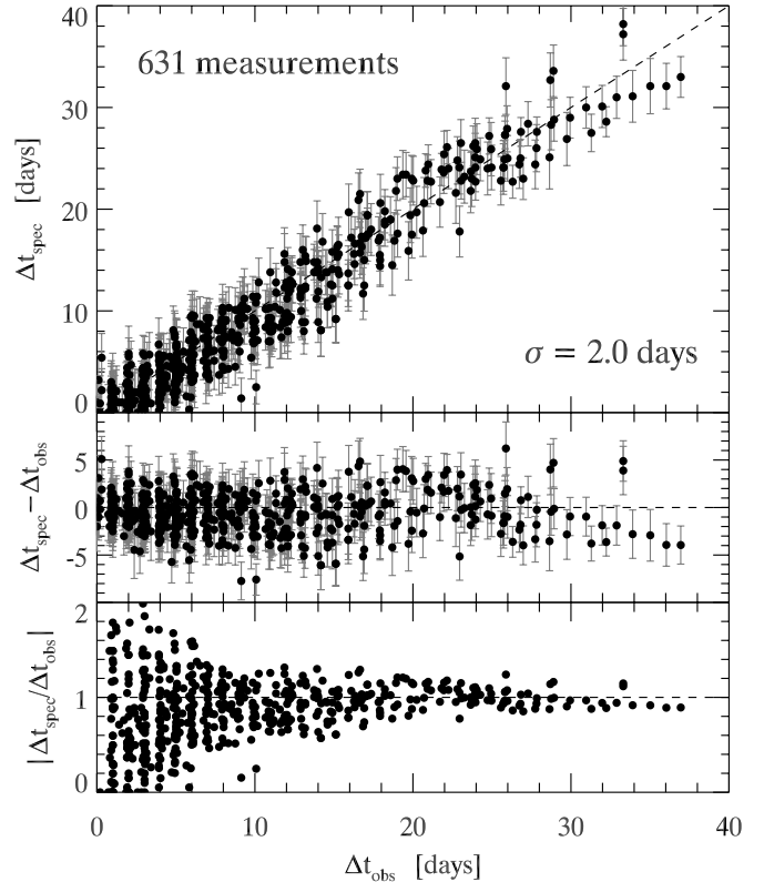
FIG. 5.— Top : Rest-frame age difference ( \Delta t_{\text{spec}} ) vs. observer-frame age difference ( \Delta t_{\text{obs}} ) for each spectrum pair for a given supernova. There are 631 such pairs, with a dispersion of 2.0 days about the one-to-one correspondence. Middle : Residuals in the top vs. \Delta t_{\text{obs}} . Bottom : Ratio of \Delta t_{\text{spec}} to \Delta t_{\text{obs}} , again vs. \Delta t_{\text{obs}} . For \Delta t_{\text{obs}} > 6 days, the fractional difference is less than 20%.
