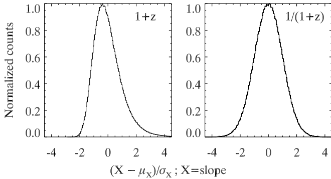
Fig. 7.— Monte Carlo results illustrating the advantage of working in 1/(1+z) space for time dilation measurements, showing recovered slope (in standard deviations from the mean, \mu ; solid lines ) in 1+z ( left ) and 1/(1+z) space ( right ), using the SN age errors reported by Foley et al. (2005). The distribution is highly non-Gaussian in the former case.
