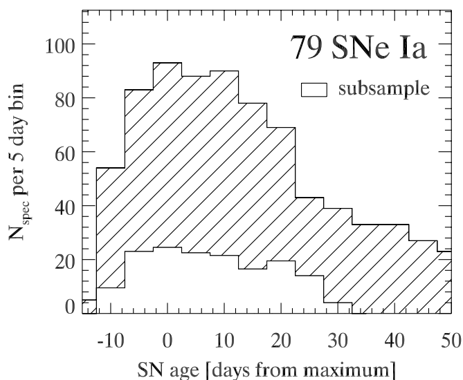
FIG. 3.—Age distribution of the 79 SN Ia templates used in SNID ( hatched histogram ). There are a total of 959 spectra with ages between -15 and +50 days from B -band maximum light. The open histogram shows the subsample of 145 spectra from 22 SNe Ia (restricted to ages between -10 and 30 days from maximum) for which we report an aging rate measurement (see § 4).
