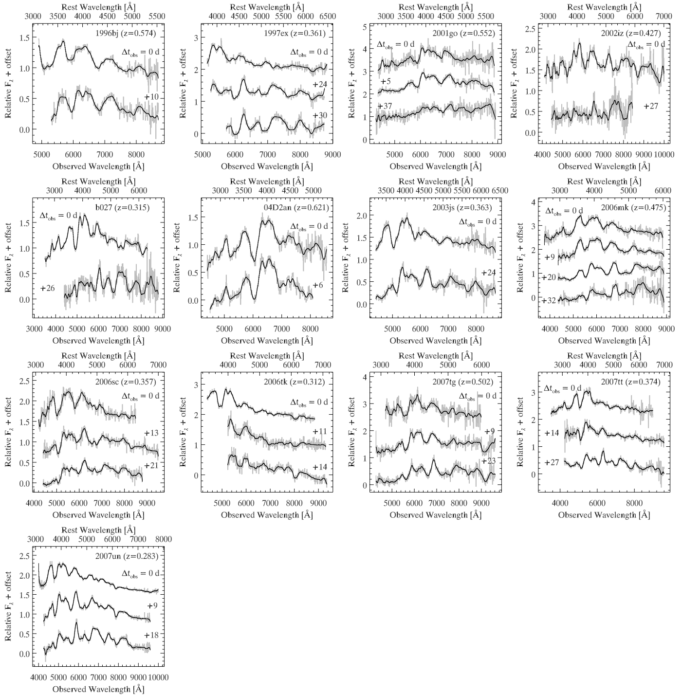
FIG. 4.—Multiepoch spectra of the 13 high-redshift SNe Ia used in this study, binned to 10 \text{ \AA} (gray). The vertical offset between the spectra is for clarity only and does not reflect differences in flux density ( F_{\lambda} ; \text{ergs s}^{-1} \text{ cm}^{-2} \text{ \AA}^{-1} ) between them. In each plot, the age of the supernova increases downward, and the observed time (in days) from the first spectrum is indicated. Overplotted in black is a smoothed version using the inverse-variance-weighted Gaussian algorithm of Blondin et al. (2006).
