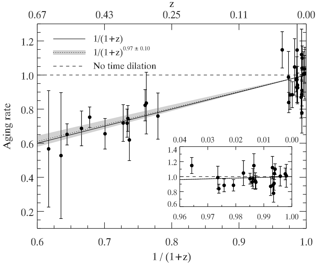
FIG. 8.— Apparent aging rate vs. 1/(1+z) for the 13 high-redshift ( 0.28 \leq z \leq 0.62 ) and 22 low-redshift ( z < 0.04 ) SNe Ia in our sample. Overplotted are the expected 1/(1+z) time dilation (solid line) and the best-fit 1/(1+z)^b model (with b = 0.97 \pm 0.10 ; dotted line and gray area). The dashed line corresponds to no time dilation, as expected in the tired-light model, clearly inconsistent with the data. Inset: Close-up view of the low-redshift sample. These data are summarized in Table 3.
