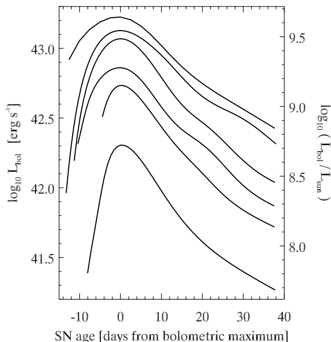
FIG. 1.—Bolometric light curves of six low-redshift SNe Ia taken from Stritzinger (2005). Top to bottom : SNe 1991T, 1999ee, 1994D, 1992A, 1993H, and 1991bg. More luminous SNe Ia have broader light curves. SN 1991bg is an example of intrinsically subluminous SNe Ia (maximum L_{\text{bol}} < 10^9 L_{\text{Sun}} ), which are less likely to be found at high redshifts.
