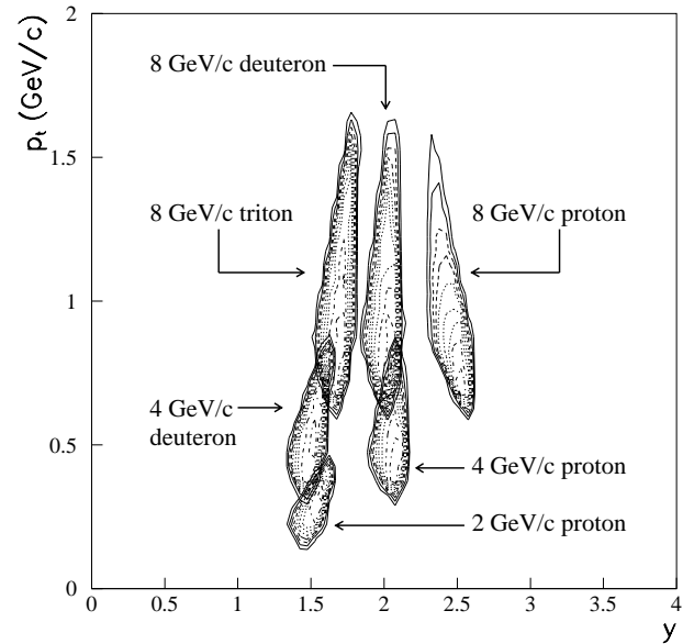
Fig. 1. The acceptance of the NA44 spectrometer at a polar angle of 129 mrad with respect to the beam direction. The acceptances are shown in p_t and y space for three different magnetic field settings corresponding to average momenta of 8, 4 and 2 GeV/c, for protons (all three settings), deuterons (8 and 4 GeV/c) and tritons (8 GeV/c)
