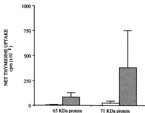
FIG. 3. The 65- and 71-kDa recombinant mycobacterial protein-induced proliferation in vitro of peripheral blood (□) and pleural effusion (▨) lymphocytes of BCG-vaccinated guinea pigs. The animals were sacrificed 1 week after induction of tuberculous pleural effusions by intrapleural injection of heat-killed M. tuberculosis cells. The mean \pm standard deviation of the mean of four to five animals per data set is shown.
